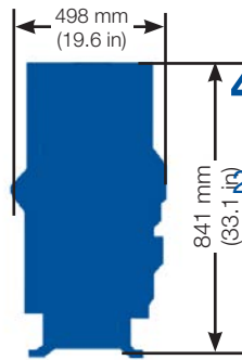
Engine package weights and dimensions
